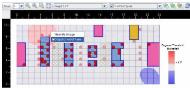
Figure 14: A hot/cold spot map. Hot air is spilling around the sides of the racks at the end of the left hand cold aisle creating a hot spot. The right mouse (context) menu shown is an extension of the MEO interface to allow interaction with the robot and its collected artifacts.
