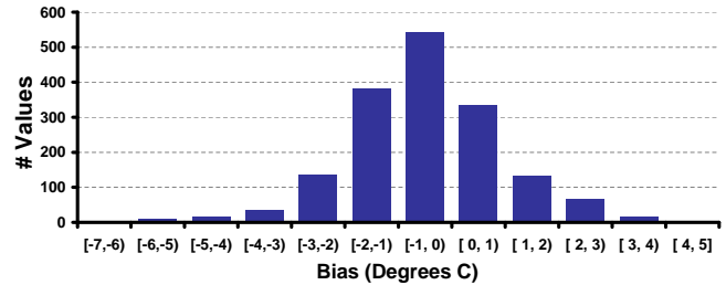
Figure 12: Interpolation bias attributable to 72 static sensors placed at 1.5 feet and 4.5 feet above the floor at both the air inlet and exhaust sides of all racks in the Poughkeepsie RC2 data center.
