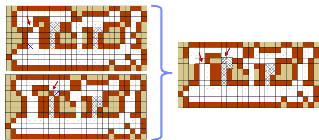
Figure 8: Example application of OR'ing to an actual data center scan. The left layouts show two scan results with misclassifications. In each layout, a key misclassification is highlighted. The right layout shows the achieved layout when OR'ing is enabled.
